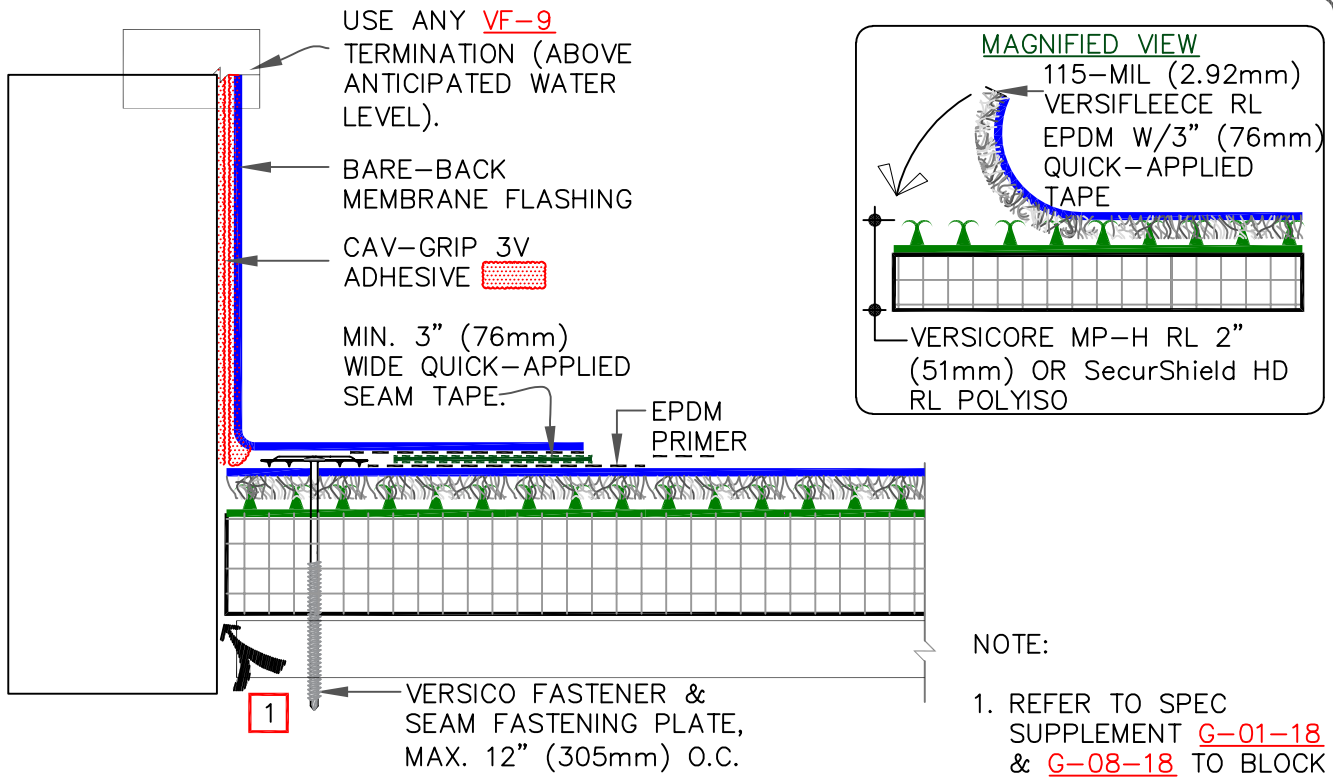
OPTION C (CAV-GRIP 3V & BARE-BACK MEMBRANE)
